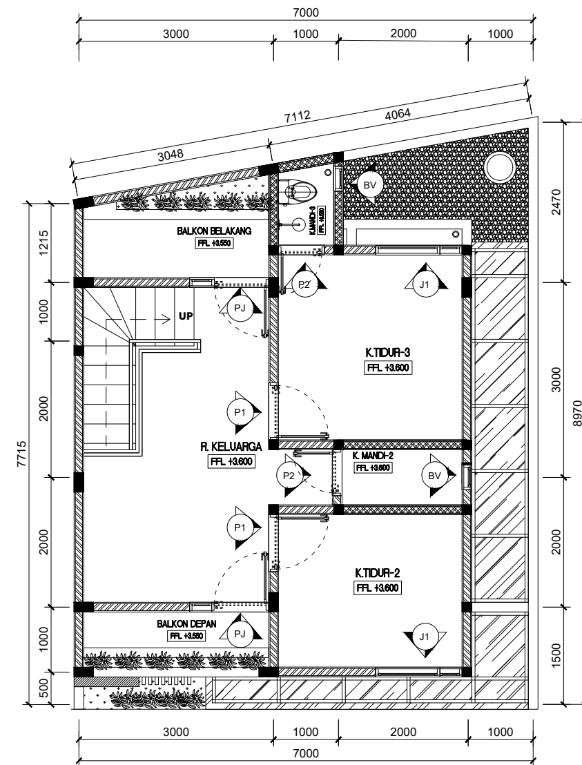
0 ARS DENAH LT.2 1:75
