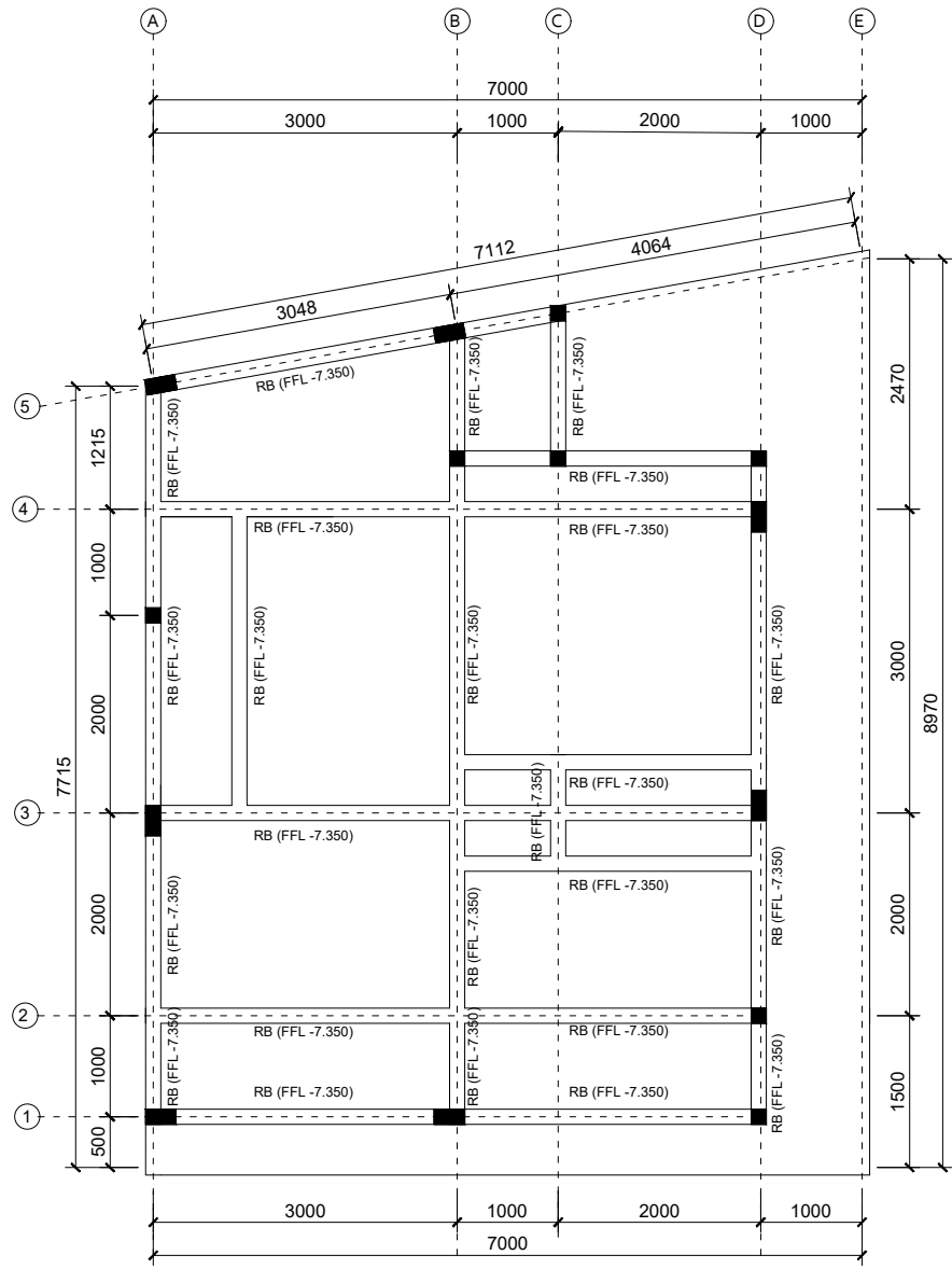
RB STR DENAH LT.2 1: 75
