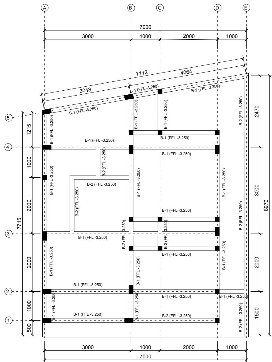
BL STR DENAH LT.1 1: 75
