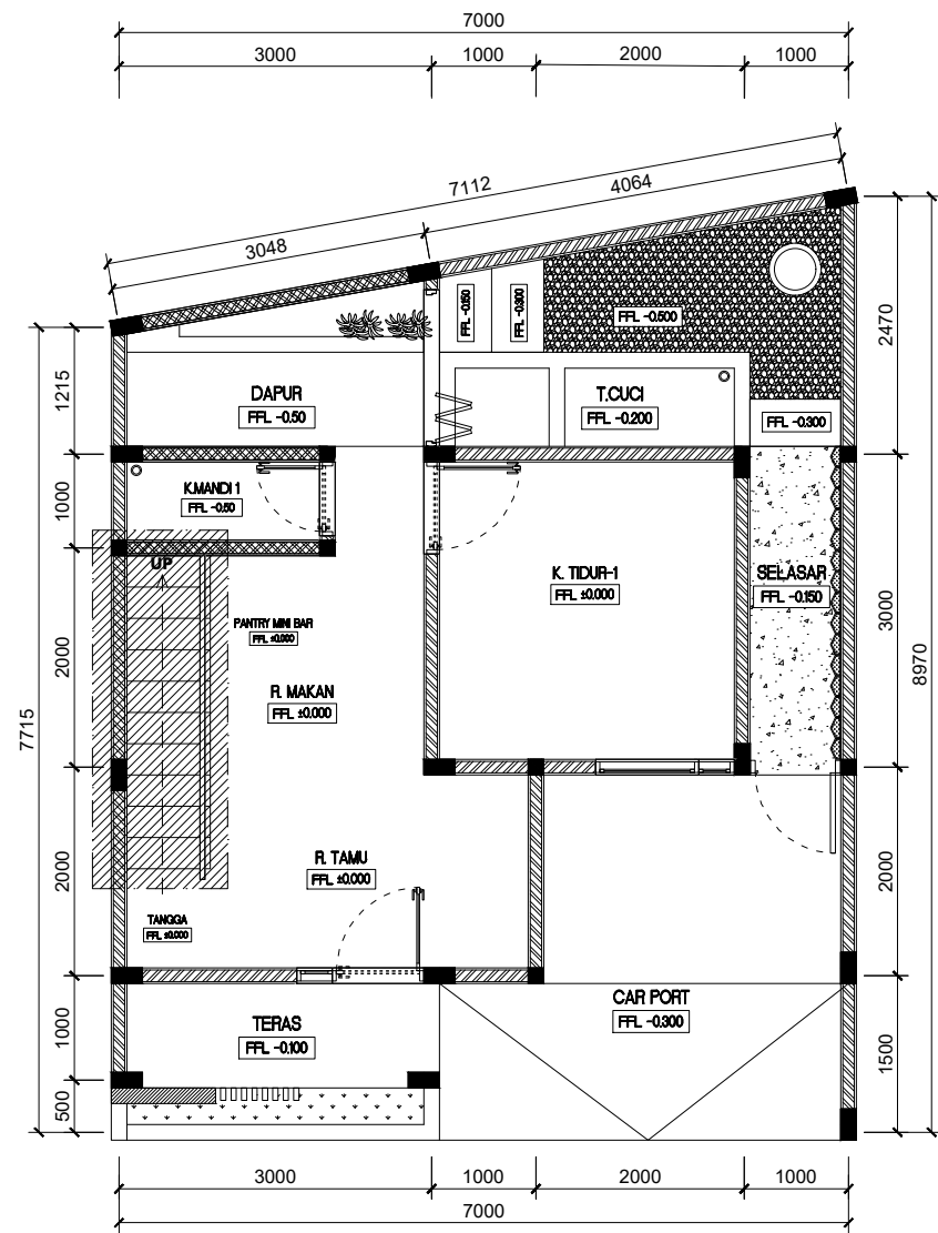
0 ARS DENAH LT.1 1: 75
