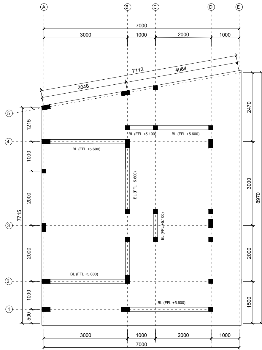
DENAH LT.2 1: 75
