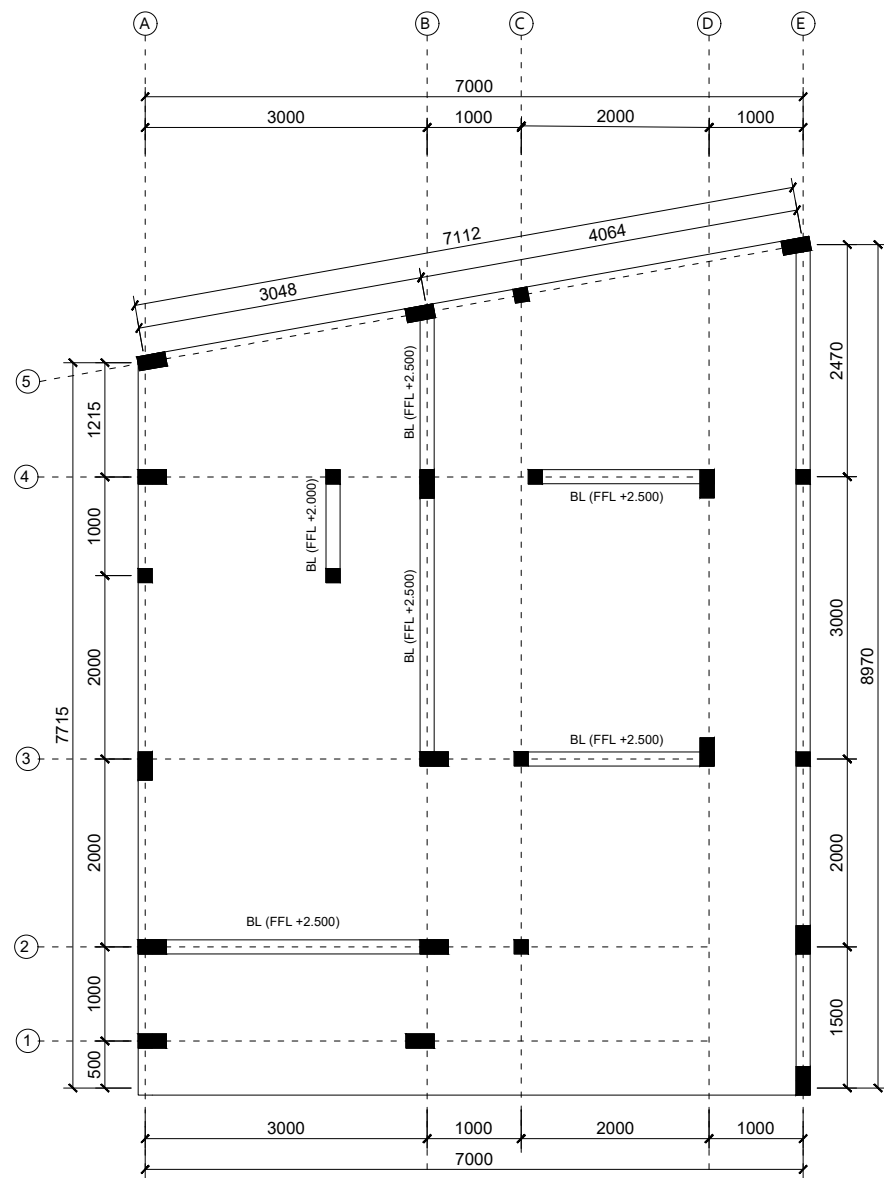
DENAH LT.1 1: 75
