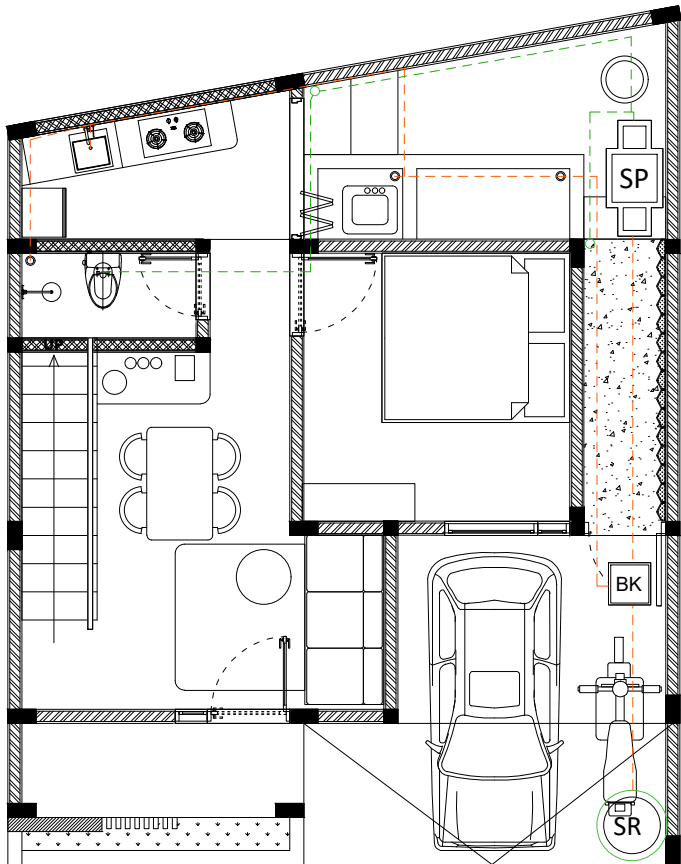
0 ME DENAH LT.1 1: 75
